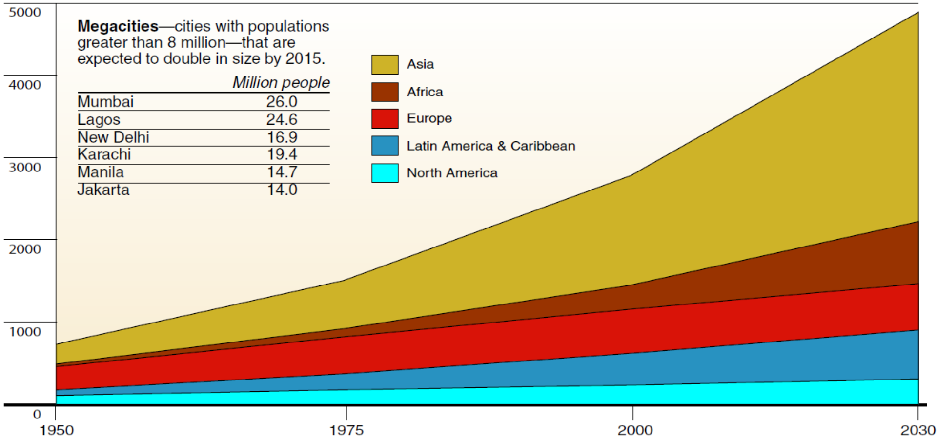
Figure 18 Urban Population by Region
